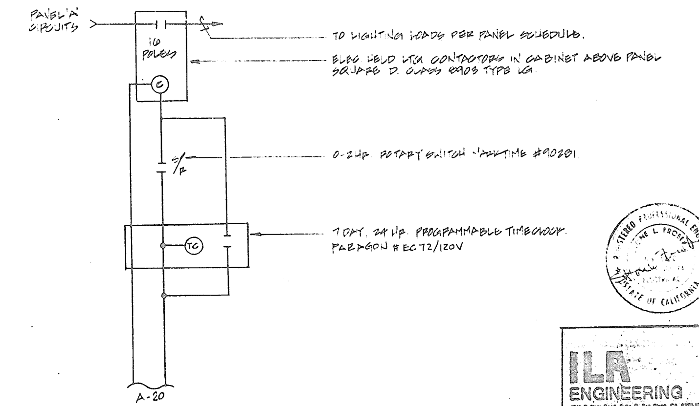
LIGHTING CONTROL WIRING DIAGRAM N.T.S.
