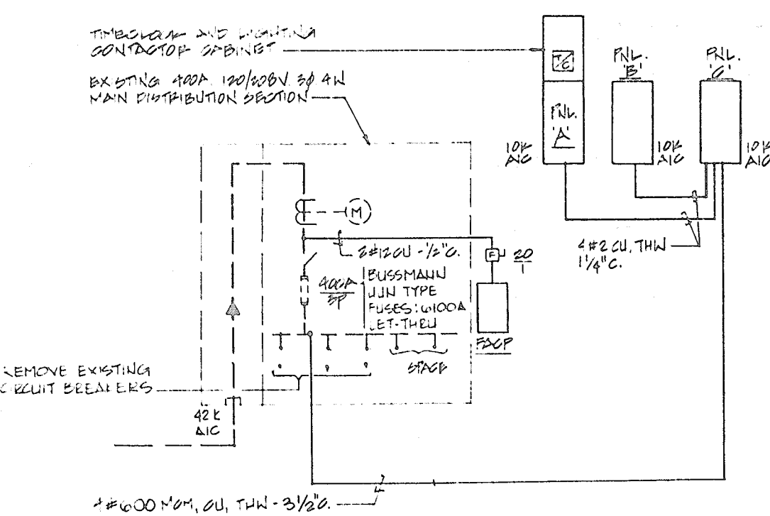
SINGLE LINE DIAGRAM N.T.S.
