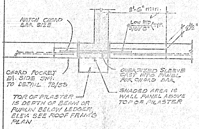
2 CHORD SPLICE @ STAND
