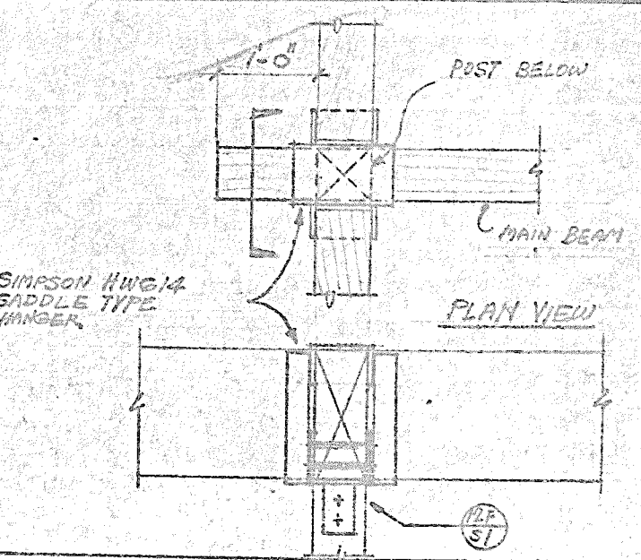
4 3-WAY BEAM CONNECT
