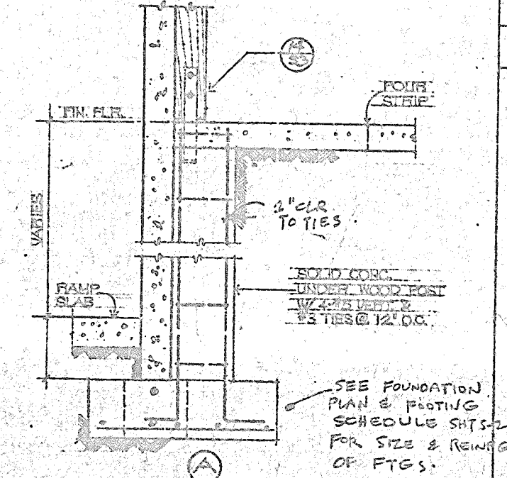
11 POST BASE AT DOCK HIGH
