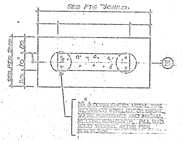
9 CONC. PIER AT ENTRY
