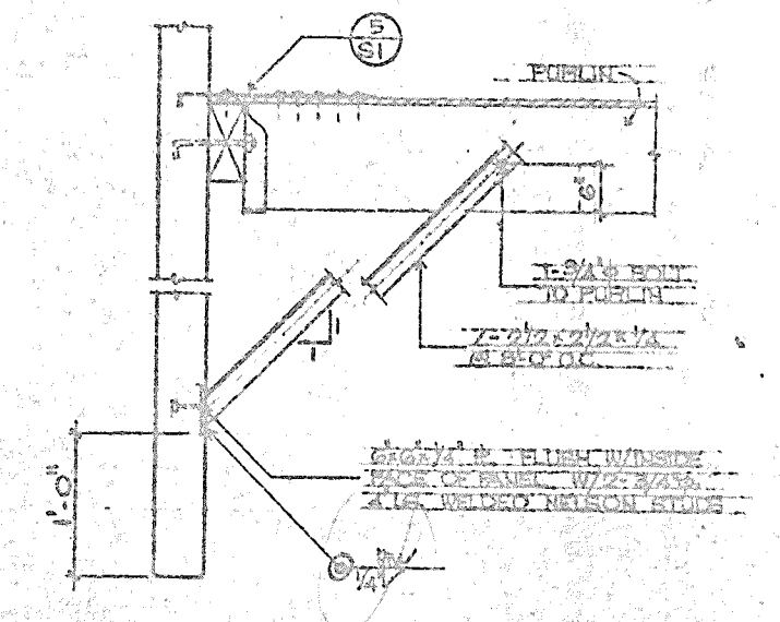
BRACE DETAIL 8
