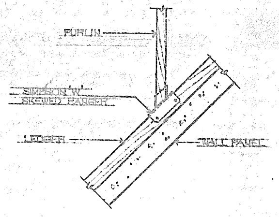
DETAIL 5
