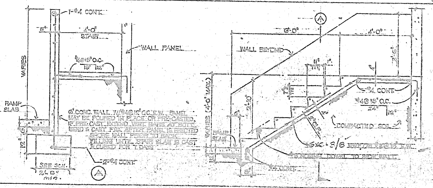
12 DRAG CONNECTION
