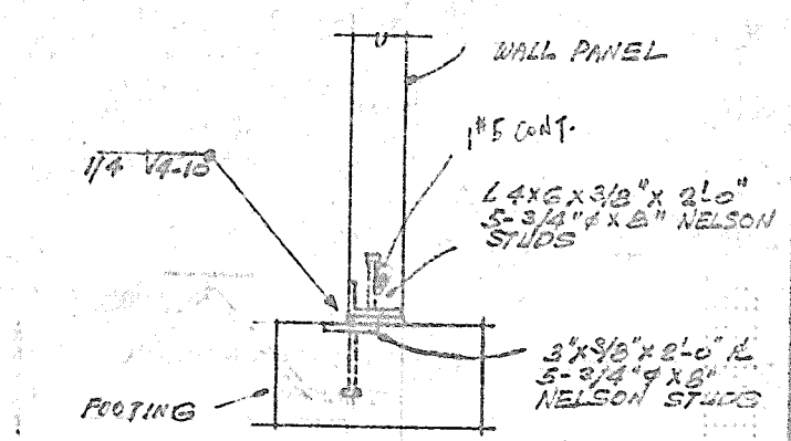
7 SHEAR ANCHOR @ WALL BASE
