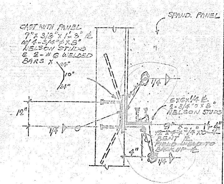
3 STAND CONNECTION
