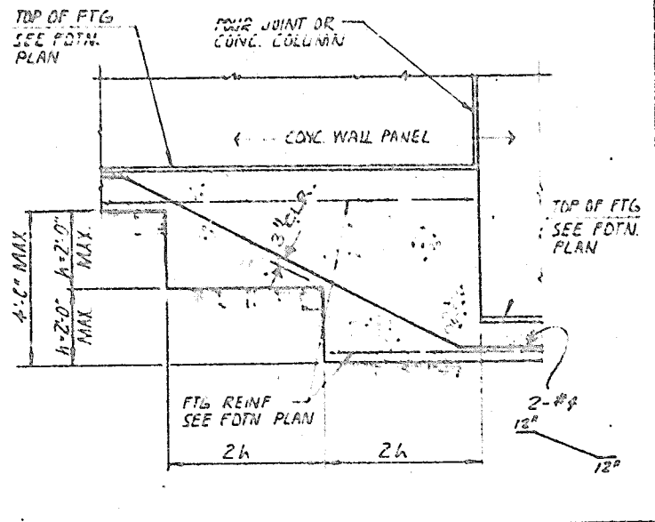
STEPPED FOOTING DETAIL
