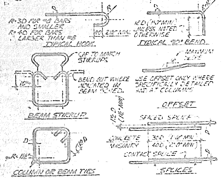
TYPICAL REINFORCING BAR BENDS
