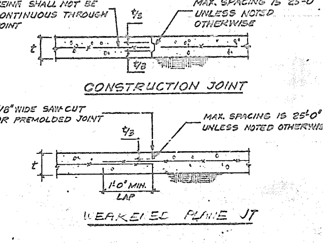
SLAB JOINT DETAILS
