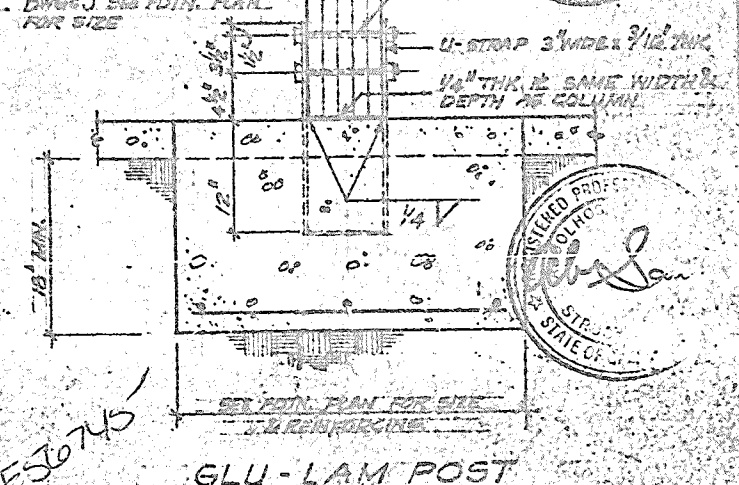
COLUMN FOOTINGS
