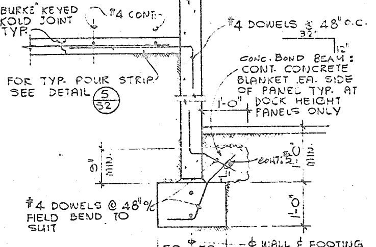
WALL SECTION
