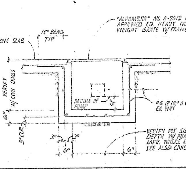
SUMP DETAIL
