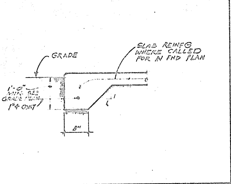
TYPICAL SLAB EDGE
