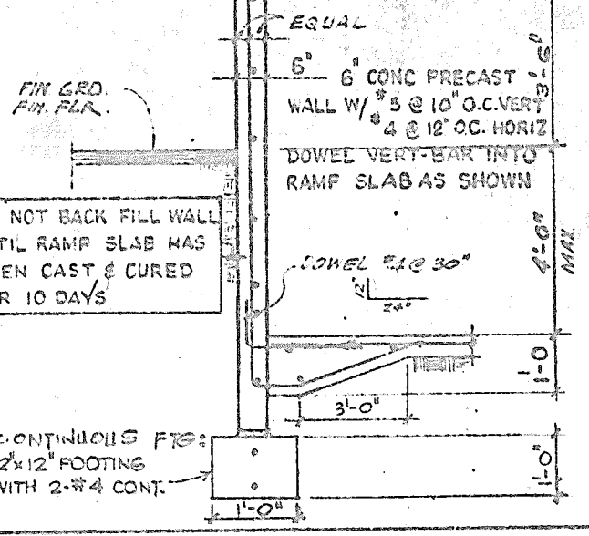
TYP. RETAINING WALL
