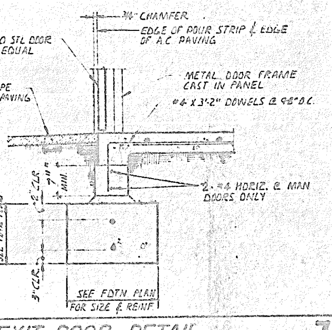
EXIT DOOR DETAIL
