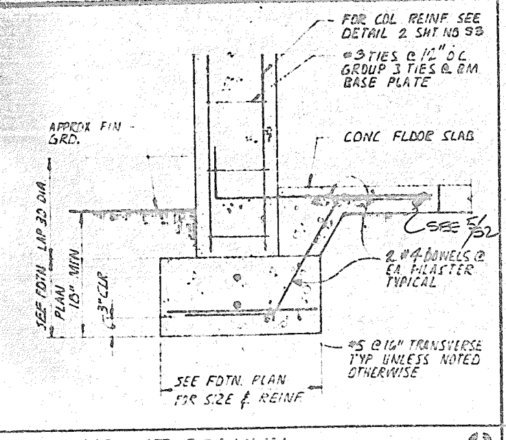
FOOTING AT COLUMN
