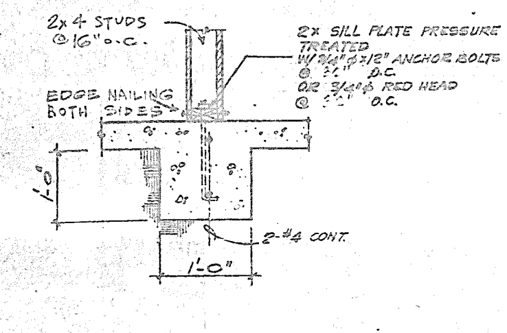
SECTION
