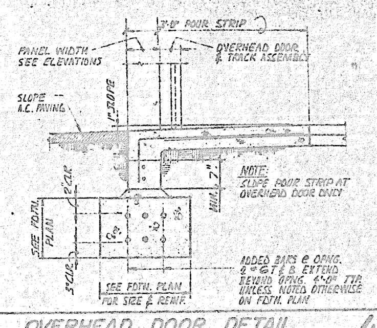
OVERHEAD DOOR DETAIL
