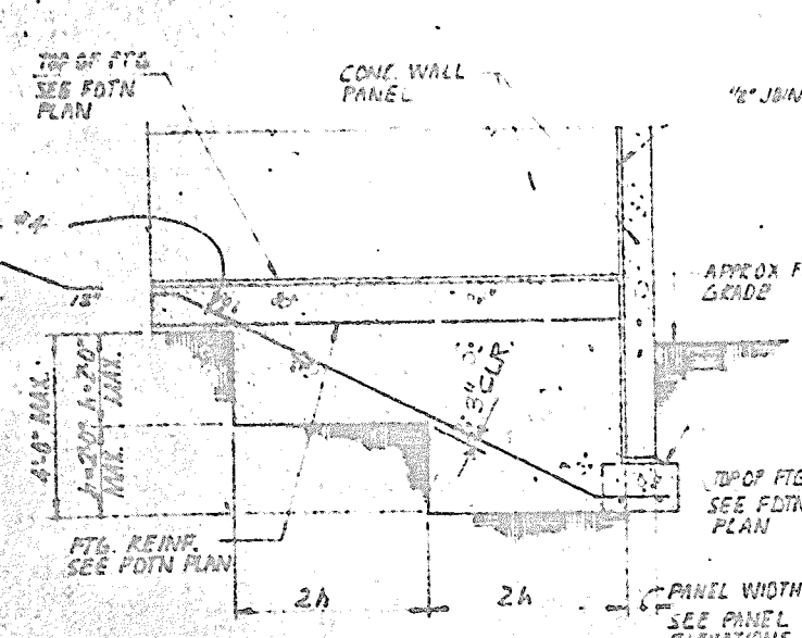
STEPPED FTG. AT CORNER
