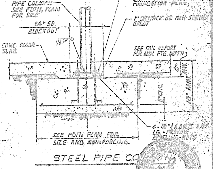
STEEL PIPE COLUMN
