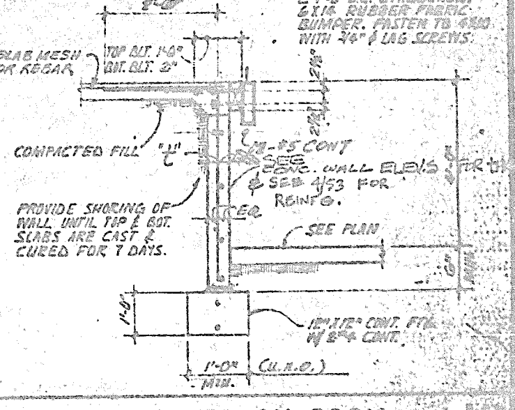
SECTION AT TRUCK DOCK
