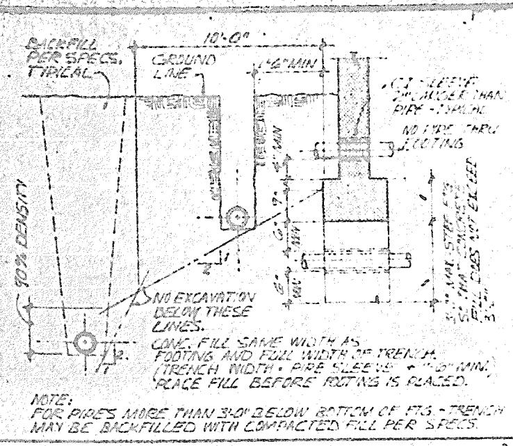
TYPICAL PIPE AT FOOTING
